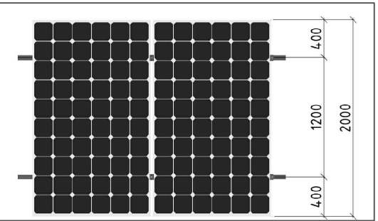
Portrait panel orientation
