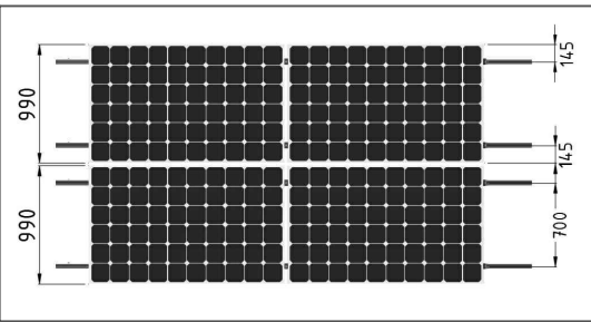
Landscape panel orientation
