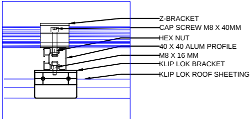
Detail E
