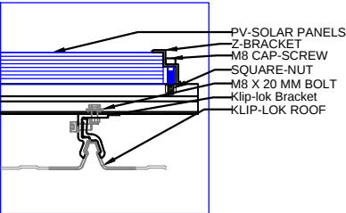
Detail D
