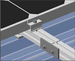
Join plate connection
