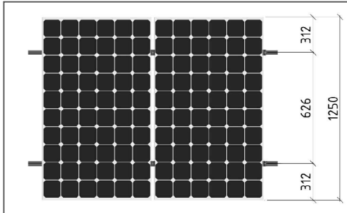
Portrait panel orientation
