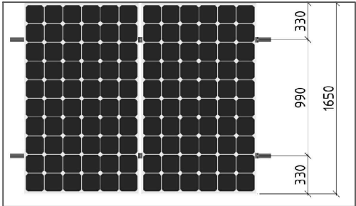
Portrait panel orientation
