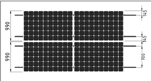
Landscape panel orientation
