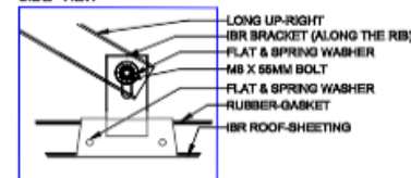
Detail C
