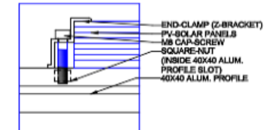
Detail E
