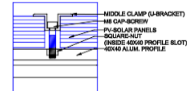
Detail D
