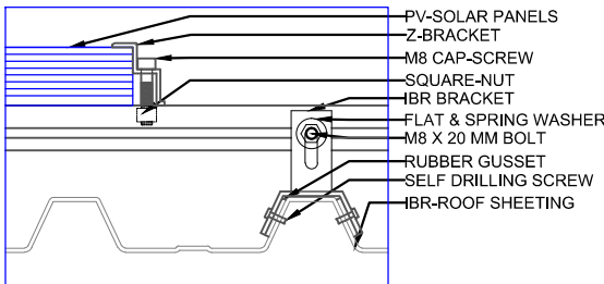
40X40 ALUMINIUM PROFILE SUPPORTING PANEL CONNECTED TO ROOF SHEET BY AN IBR BRACKET (FRONT-VIEW)
