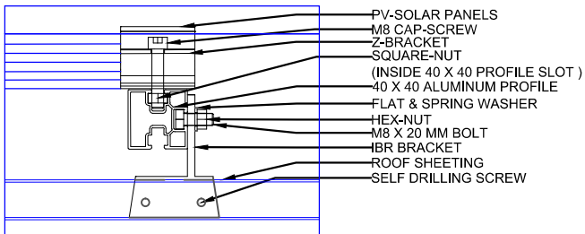
40X40 ALUMINIUM PROFILE SUPPORTING PANEL CONNECTED TO ROOF SHEET BY AN IBR BRACKET (SIDE-VIEW)
