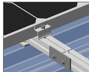
Join plate connection
