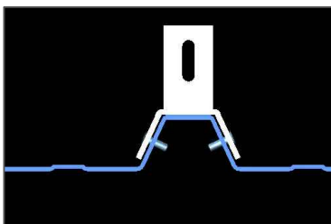
IBR Bracket going along with self drilled screws (front-view)
