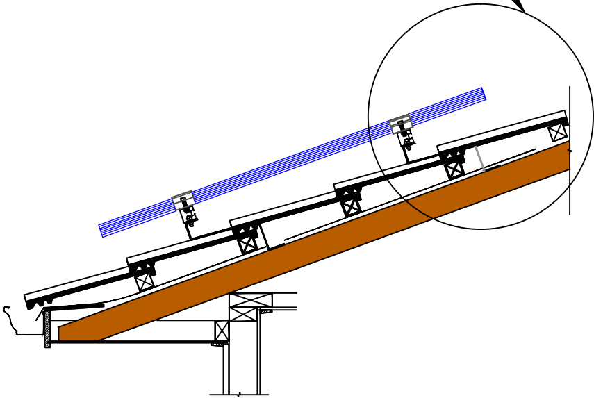
DETAIL A
