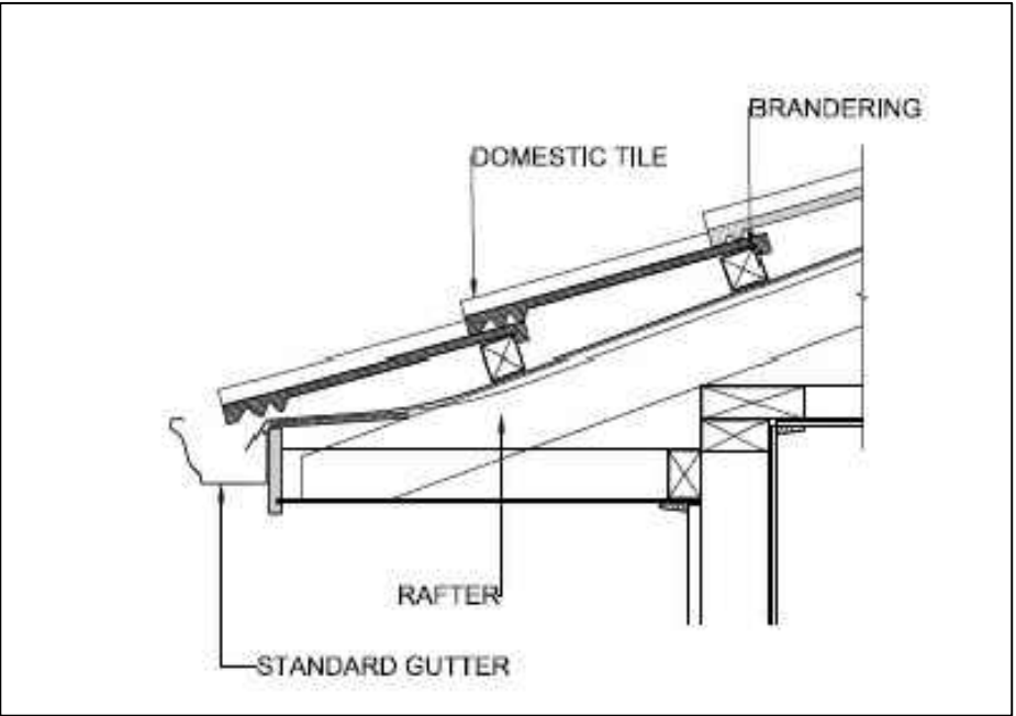
INTERNAL SIDE-VIEW
