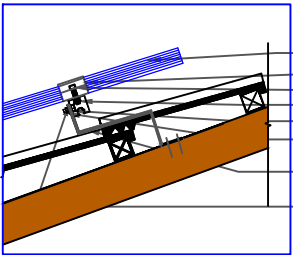
Domestic tile roof bracket supporting 40 x 40 Alum. with top and side fixing
