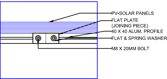
TWO 40X40 ALUMINIUM PROFILES ACTING AS ONE JOINED TOGETHER BY A FLAT PLATE
