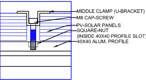
Middle clamp (U-bracket) holding panels and connecting to profile
