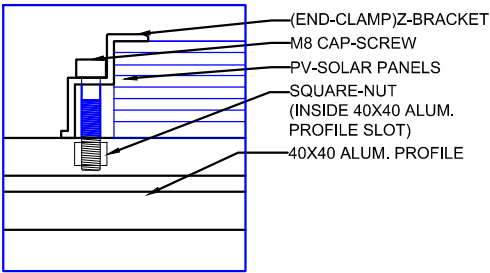
End clamp (Z-Bracket) holding panels and connecting to Aluminum profile
