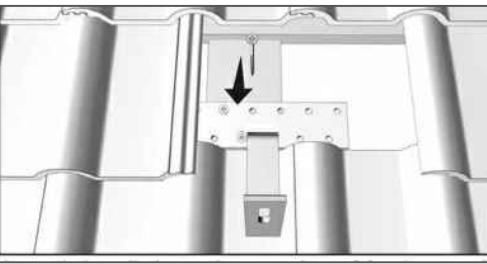
Installed domestic bracket
