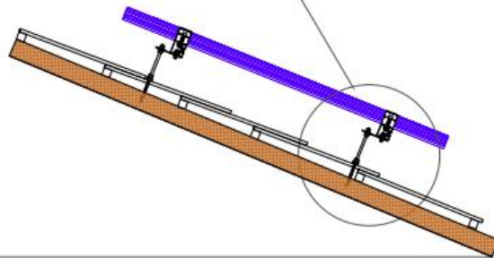
Hanger Bolt
