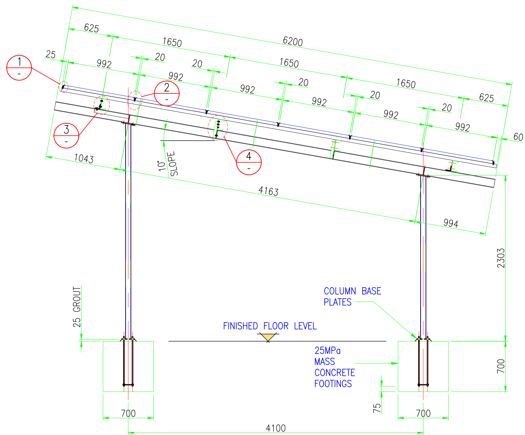
SIDE ELEVATION
