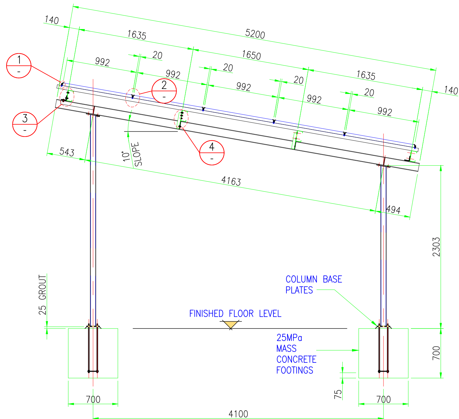
SIDE ELEVATION
